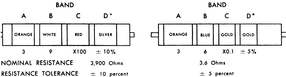
Figure 4-9. Color code marking for MIL-STD resistors.
