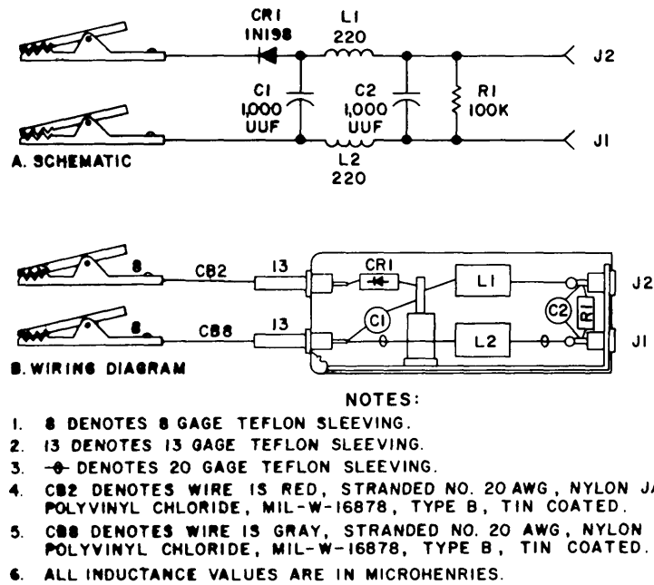
Figure 4-6. Neutralizing detector, schematic and wiring diagram.
