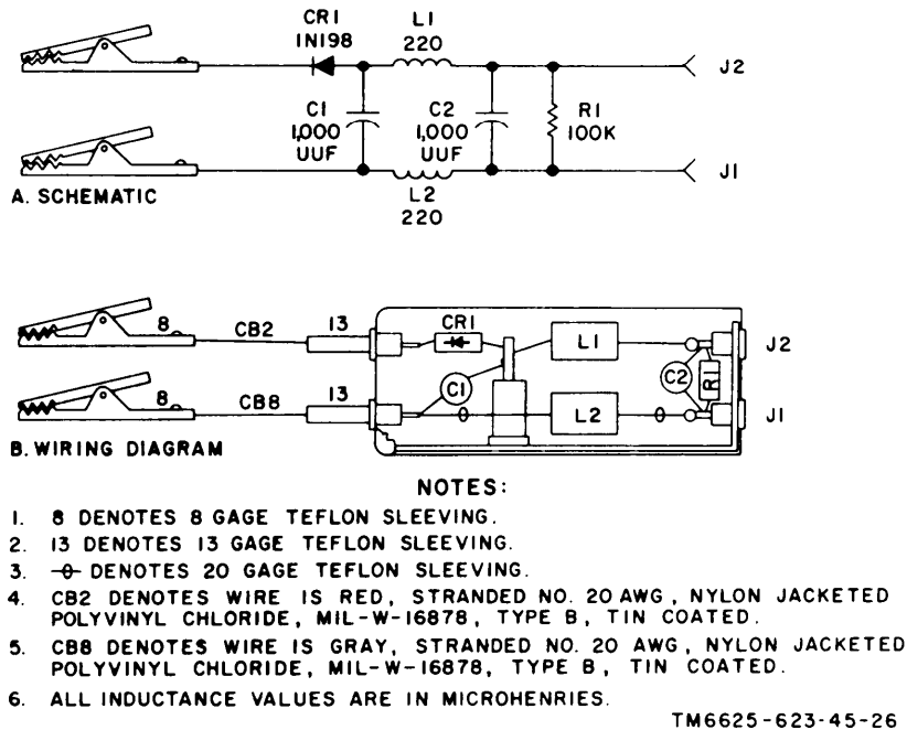
Figure 4-6. Neutralizing detector, schematic and wiring diagram.
