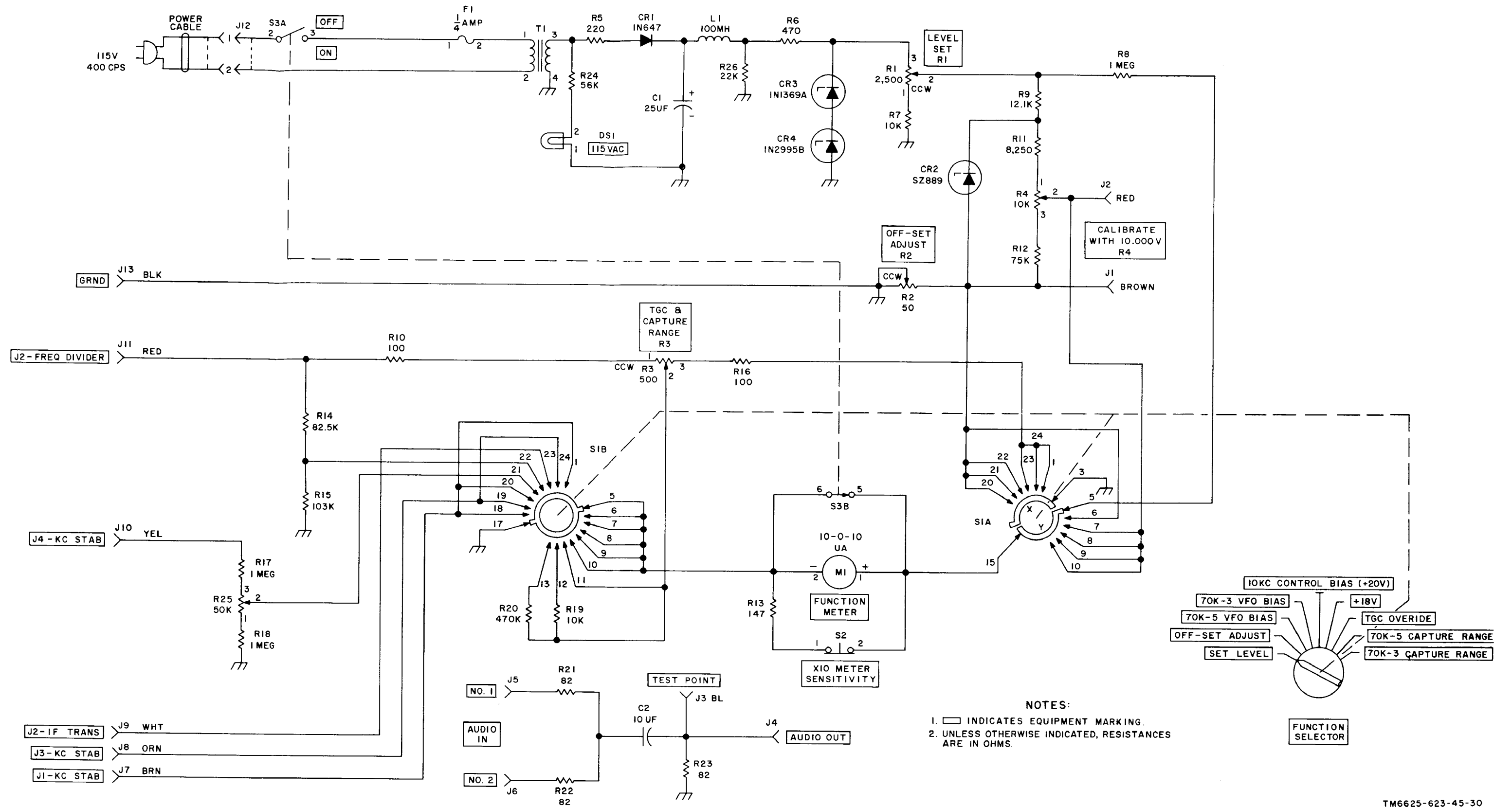
Figure 4-11. Function test set, schematic diagram.
