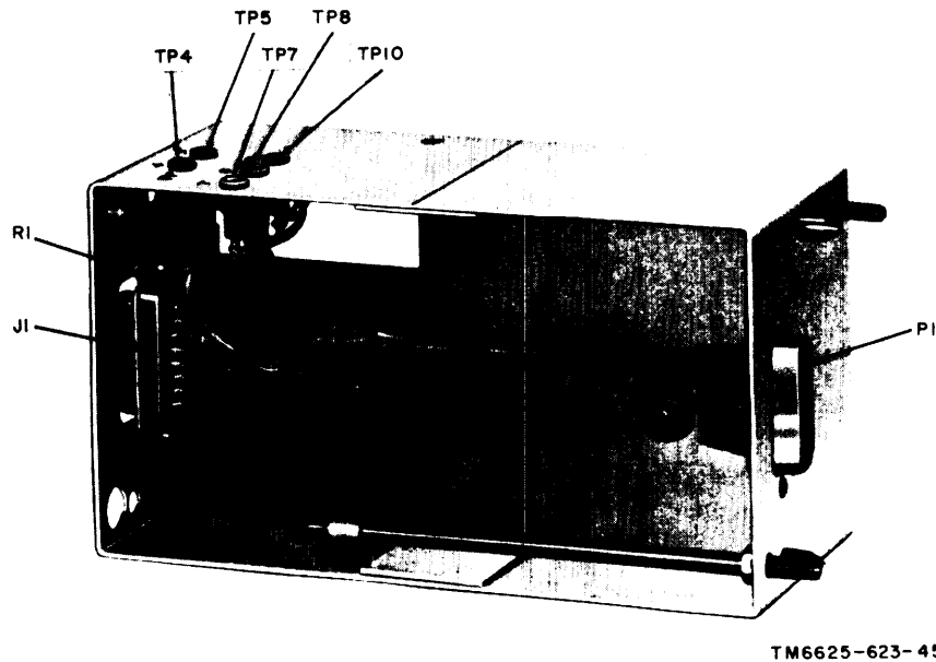
Figure 3-15. Low-voltage power supply module extender, parts location.
