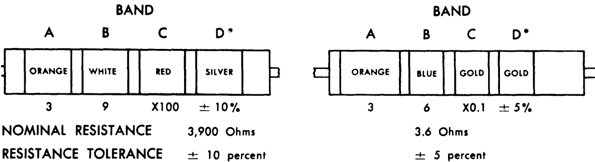
Figure 4-9. Color code marking for MIL-STD resistors.
